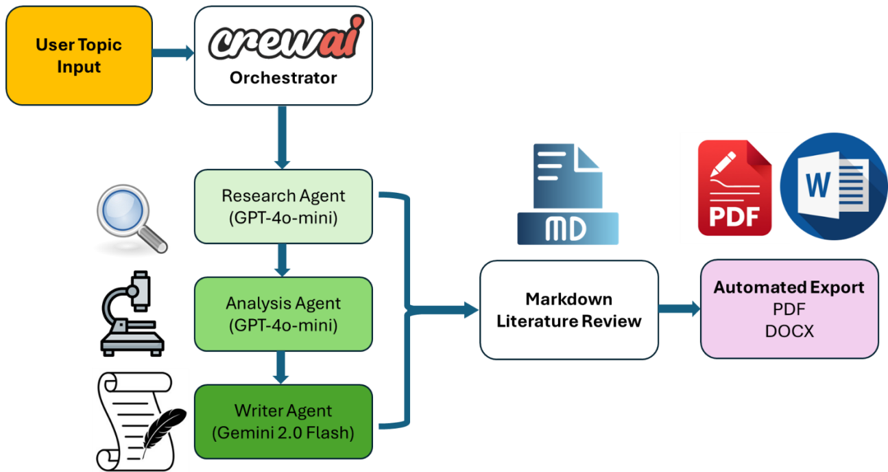
Schematic of the CrewAI Multi-Agent Pipeline for Hydrology-focused Literature Review
